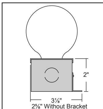
CROSS SECTION
